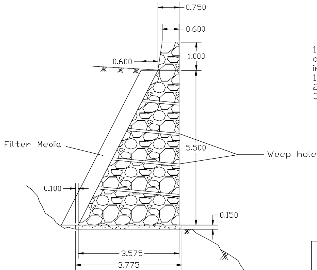
TCS-3 : Typical Cross Section of RR Masonry Retaining Wall
